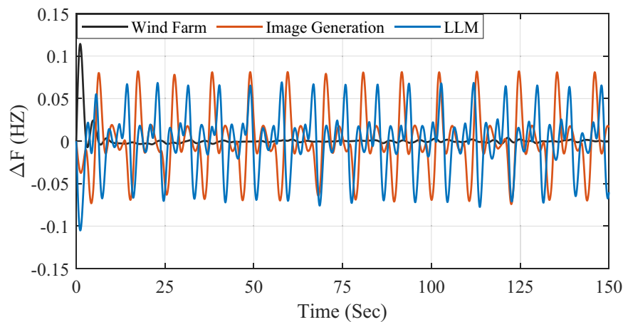
Fig. 14 AGC frequency variation under wind farm generation, AI image generation training workload and, AI LLM training workload.
