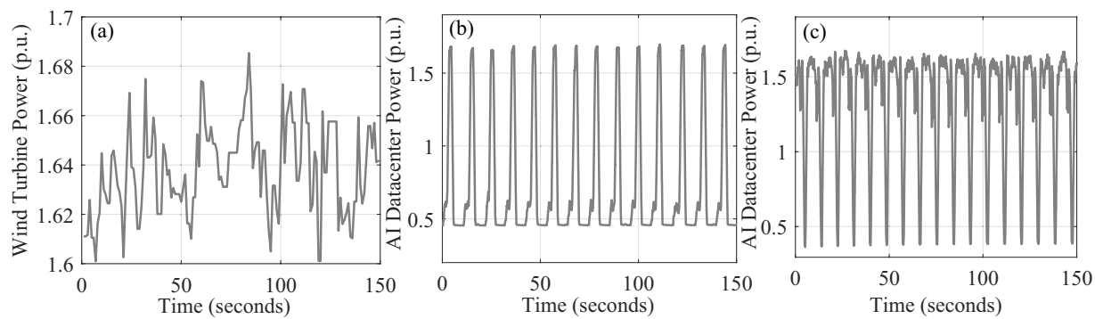
Fig. 13 Area 1 power profiles under different operating scenarios: (a) wind farm generation, (b) AI image generation training workload, and (c) AI LLM training workload.
