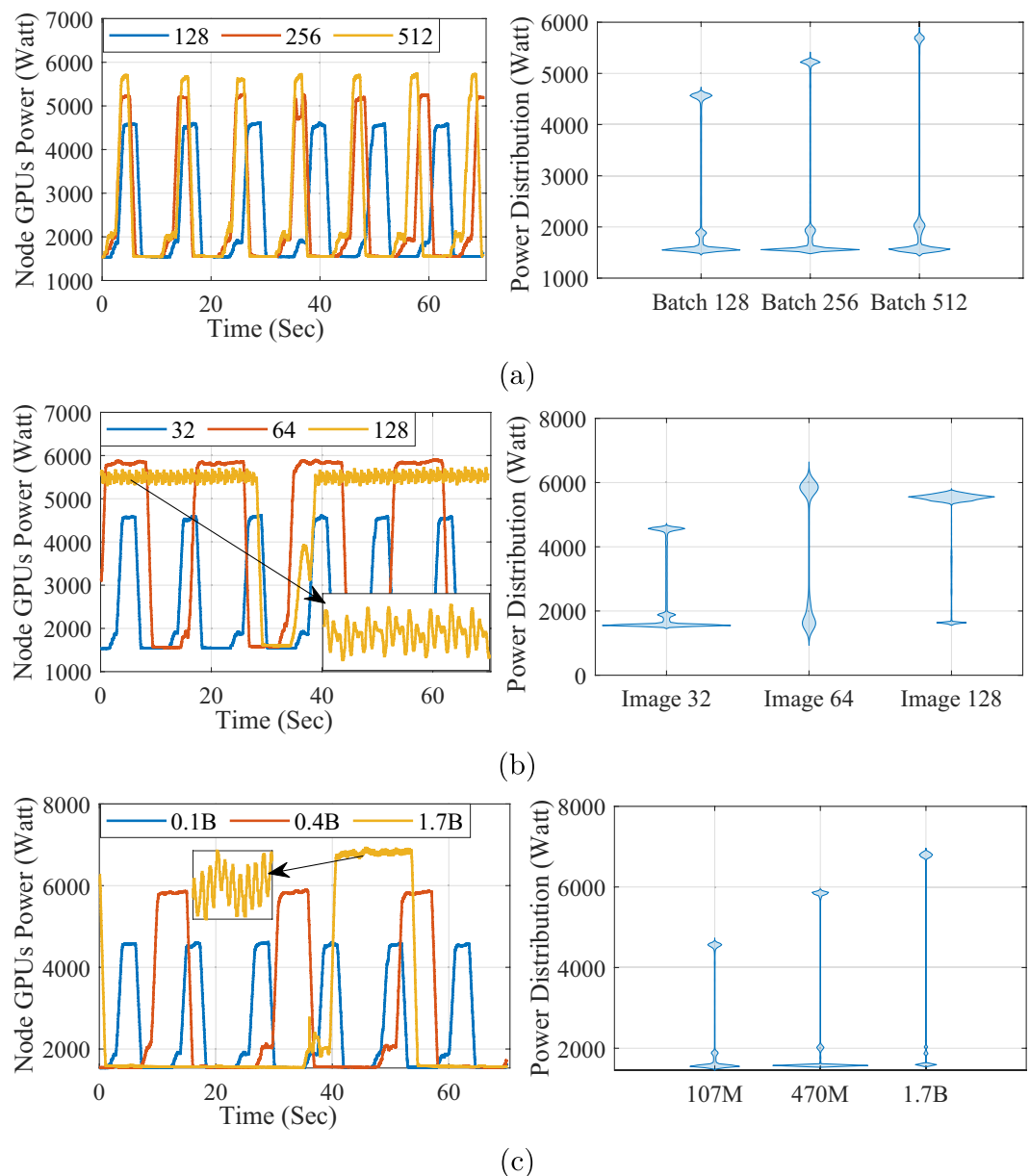
Fig. 10 Correlation and power trends in a multi-GPU node under varying AI model architectures and hyperparameters during image generation training using a diffusion model on a B200 node: (a) batch size, (b) image size, and (c) model size.
