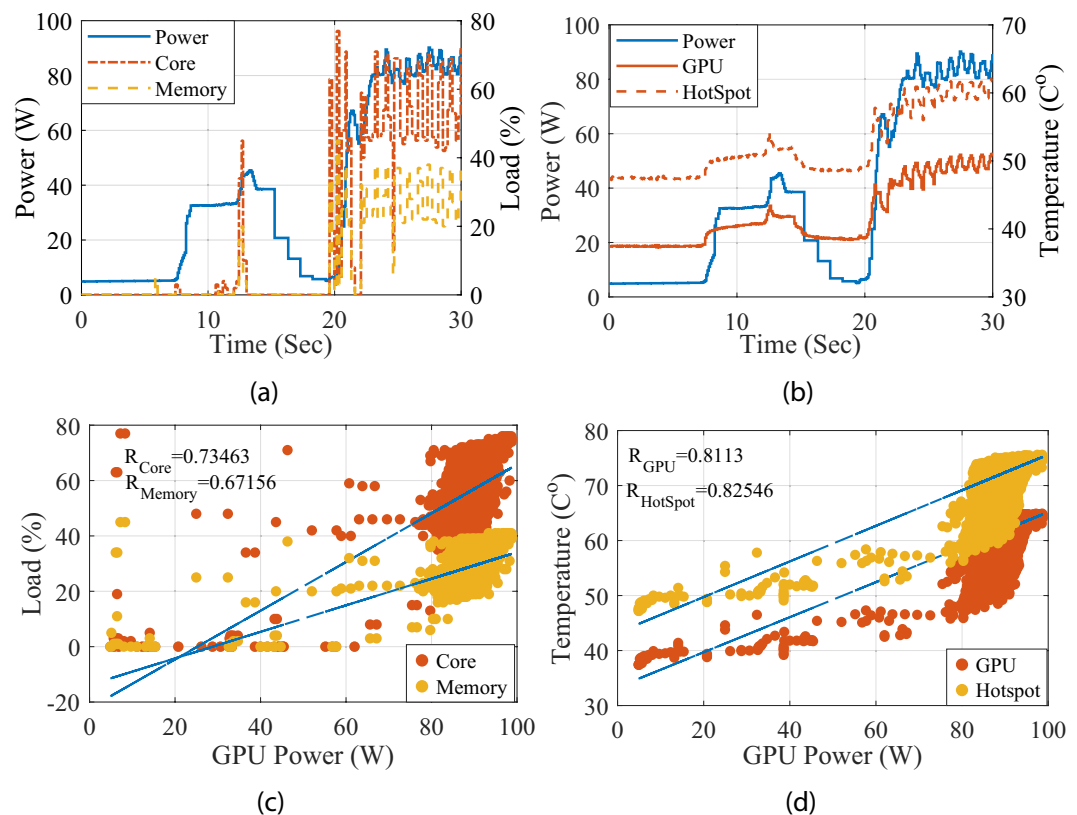
Fig. 8 GPU performance metrics correlation, (a) GPU power, core, and memory load temporal evolution, (b) GPU power, temperature, and hotspot temperature temporal evolution, (c) GPU power and load correlation, and (d) GPU power and temperature correlation.
