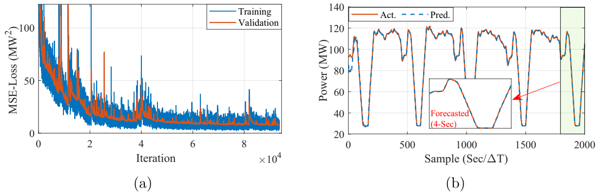
Fig. 15 Short-term time-series forecasting results using LSTM-DNN model (a) training performance, (b) testing performance on new batch. The historical window is set for 40 seconds and forecasting window for 4 seconds.
