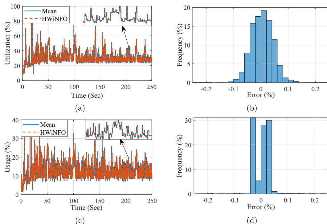
Fig. 6 CPU Utilization and Usage consistency: (a) Total CPU utilization using mathematical calculation and HWiNFO reported values, (b) corresponding utilization error, (c) Total CPU usage using mathematical calculation and HWiNFO reported values, and (d) corresponding usage error.
