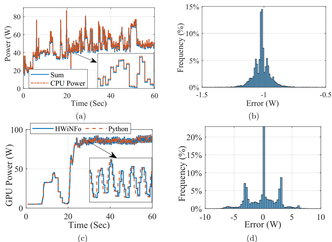
Fig. 5 CPU and GPU measurement consistency: (a) CPU package power compared with the sum of core, GT core, system agent, and Rest-of-Chip power components, (b) corresponding sum error, (c) GPU power monitoring using HWiNFO and Python monitoring code, and (d) corresponding matching error.
