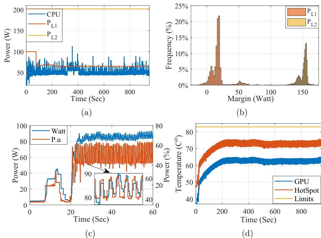
Fig. 3 Operation Limits, (a) CPU power and dynamic power demand limits, (b) power margin distribution, (c) GPU power and percentage loading, and (d) GPU temperature with thermal limits analysis.
