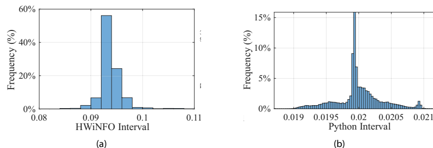
Fig. 2 Distribution of reporting intervals for (a) HWiNFO, and (b) Python monitoring tools.
