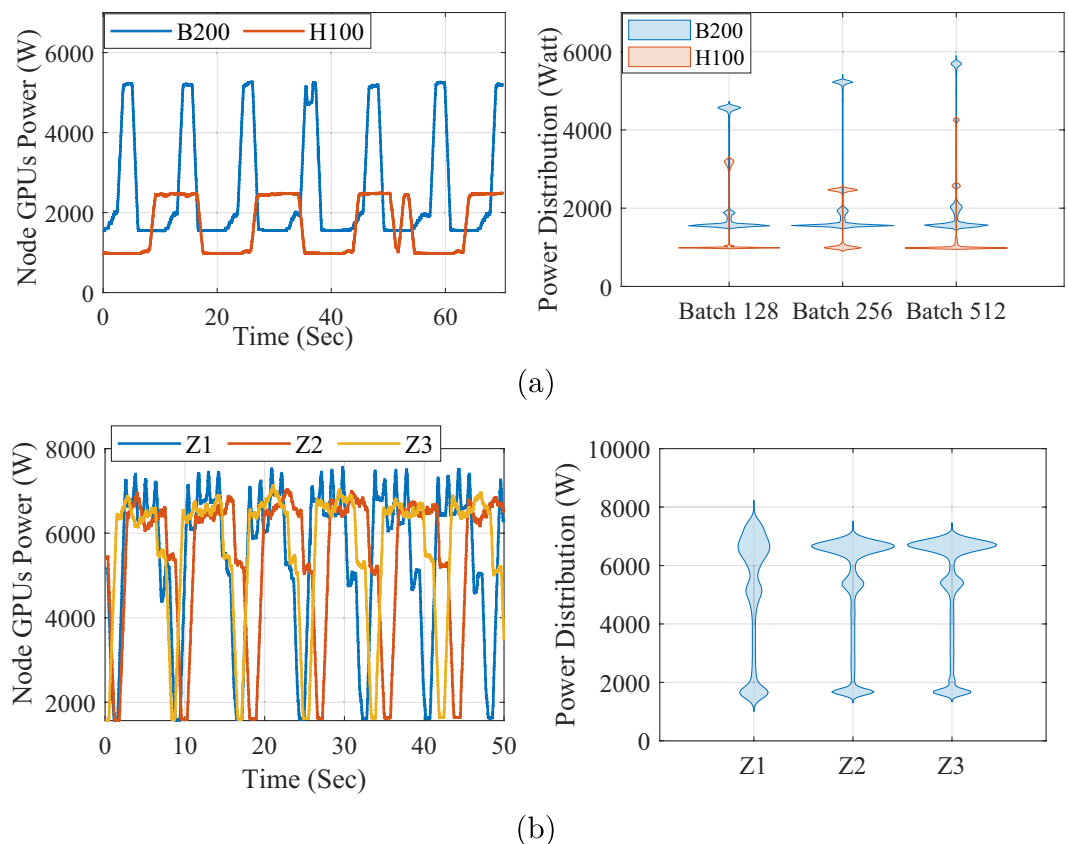
Fig. 11 Power and correlation characteristics of a text generation workload in a multi-GPU node under varying node capabilities and parallelization configurations: (a) different hardware types and (b) parallelization settings using an LLM on a B200 node.
