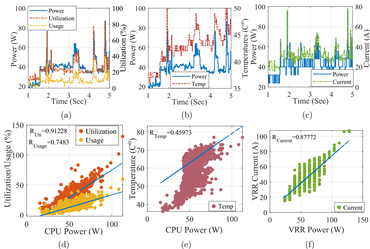
Fig. 7 CPU performance metrics correlation: (a) power-utilization time series, (b) power-temperature time series, (c) power-current time series, (d) power-utilization correlation, (e) power-temperature correlation, and (f) power-current correlation.
