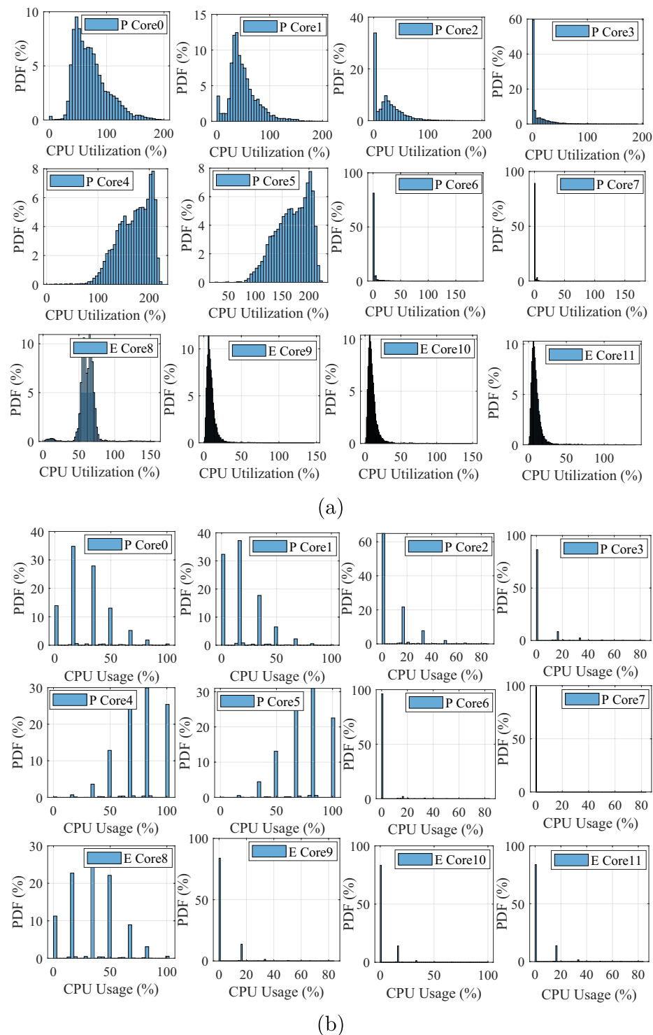
Fig. 4 CPU core utilization and usage matrix (a) The CPU cores utilization lies within the expected operation range of 233.33%, (b) The CPU cores usage lies within the expected operation range of 100%.
