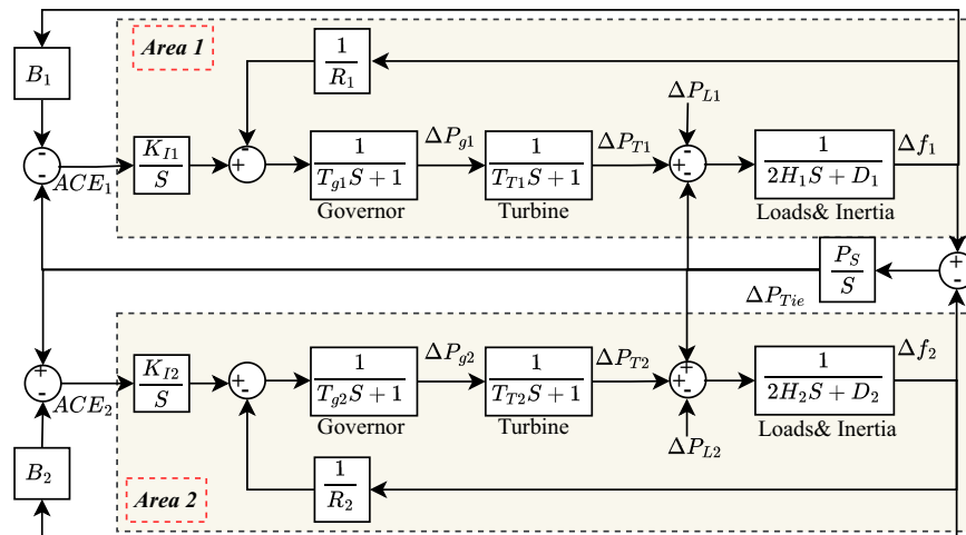
Fig. 12 Block Diagram of a 2-area AGC system for AI datacenter connection impact assessment.
